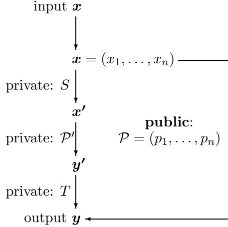
Figure 2: \mathcal{MQ} -trapdoor (S, \mathcal{P}', T) in STS
