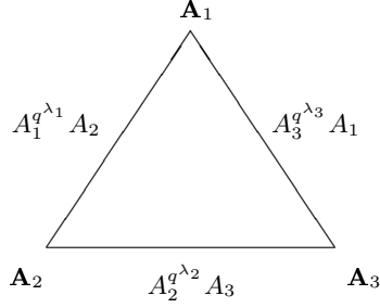
Figure 2. Graphical Representation of 3-Invertible Cycles
